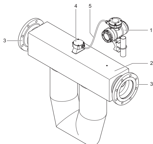
Fig. 6: Configuration of the Rotamass remote type
